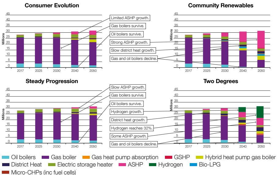
Figure 4.14 Heating technologies by scenario
