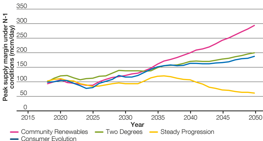
Figure 5.17 Peak gas supply margin under N-1 conditions
