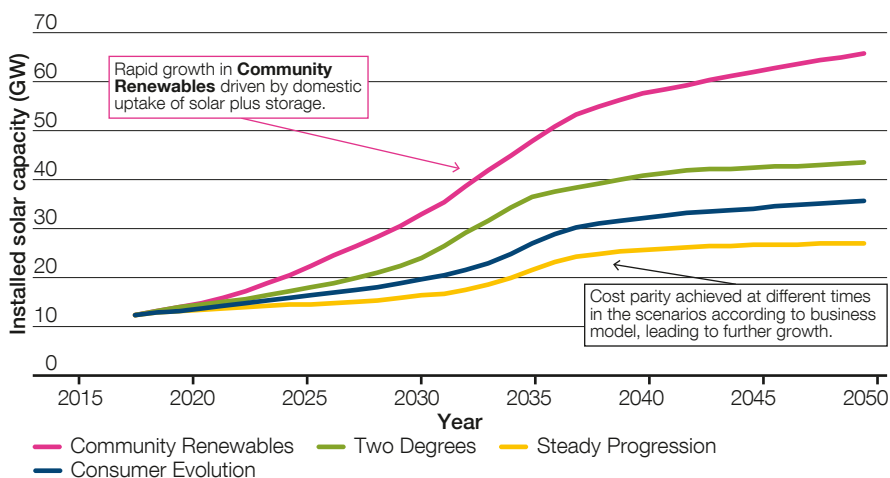
Figure 5.4 Solar capacity
