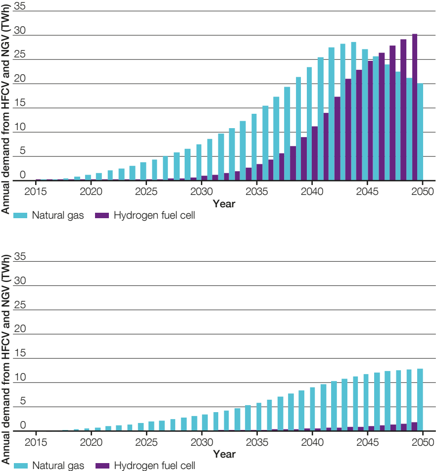
Figure 4.20 Annual demand from hydrogen fuel cell vehicles (HFCV) and natural gas vehicles (NGV) for Community Renewables (top) and Steady Progression (bottom)
