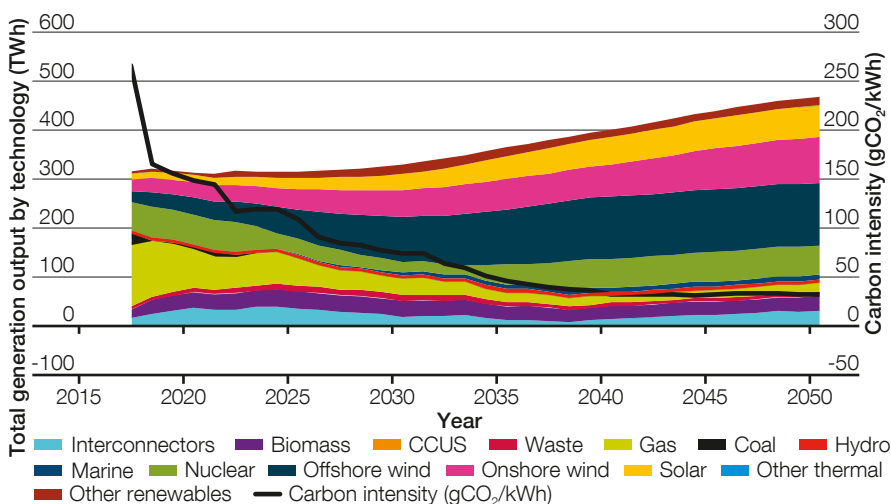
Figure 5.2 Electricity output and carbon intensity of electricity, Community Renewables scenario
