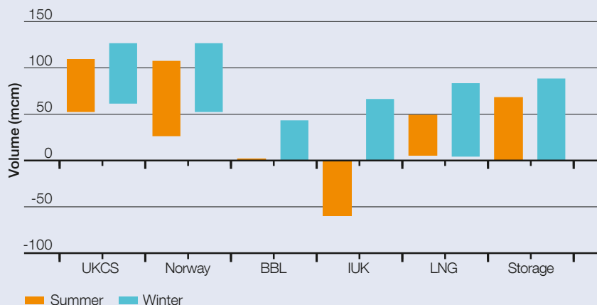
Figure 5.16 Range of daily gas supply volumes in winter and summer 2017–2018
