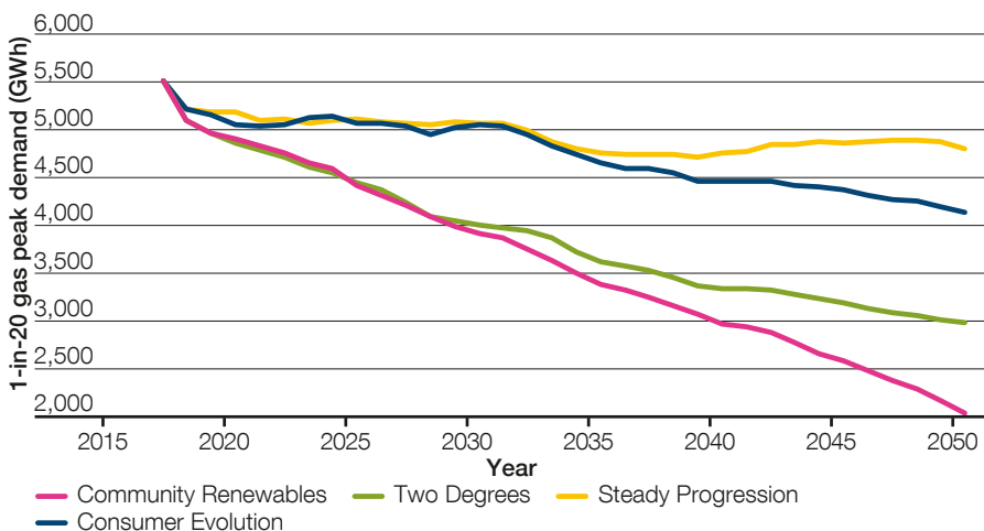
Figure 4.3 Gas 1-in-20 peak demand
